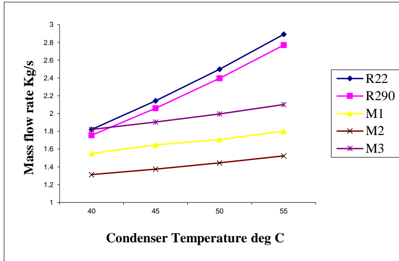
Fig 1 Variation of mass flow rate with condenser temperature
